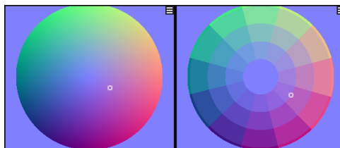
Figure 260: Aseprite's normal mapping color picker (both in its normal and discrete versions)
